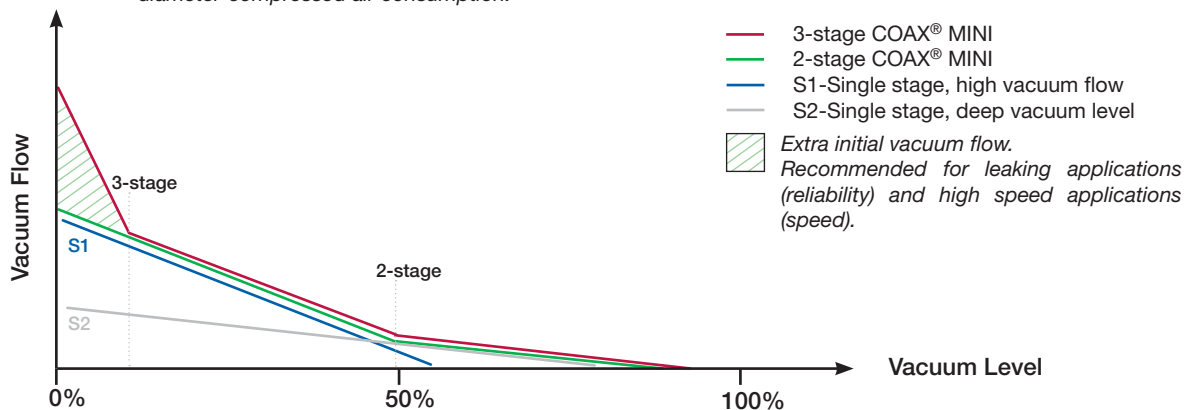
The graphs represent ejectors that are equal in nozzle diameter-compressed air consumption.
