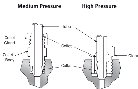
Structure of an anti-vibration screw connection
