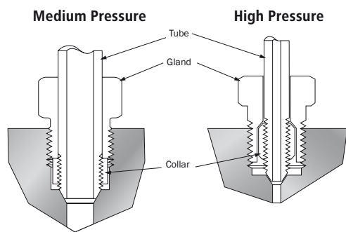
Structure of a high-pressure screw connection
