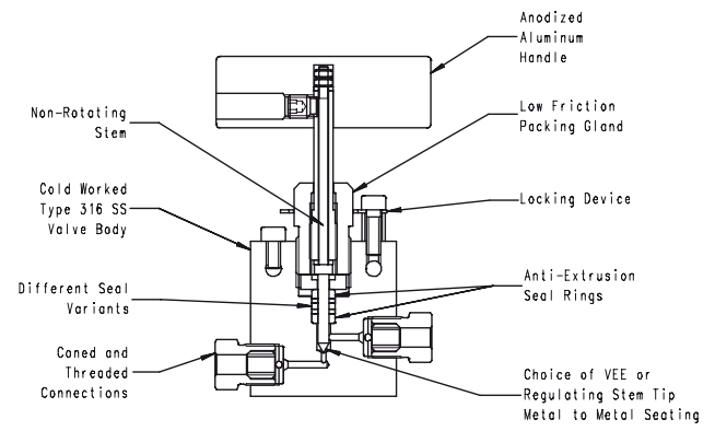
Valve Shown: 65V4H071
