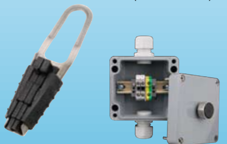
Cable clamp Art. no. 20636 JunctionBox FMD(IP67) Art. no. 20069
