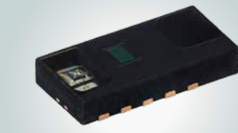
VCNL4020X01 Integrated Proximity and Ambient Light Sensor
